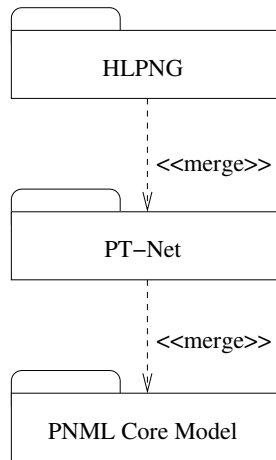
Figure 1: Overview on the UML packages of PNML
