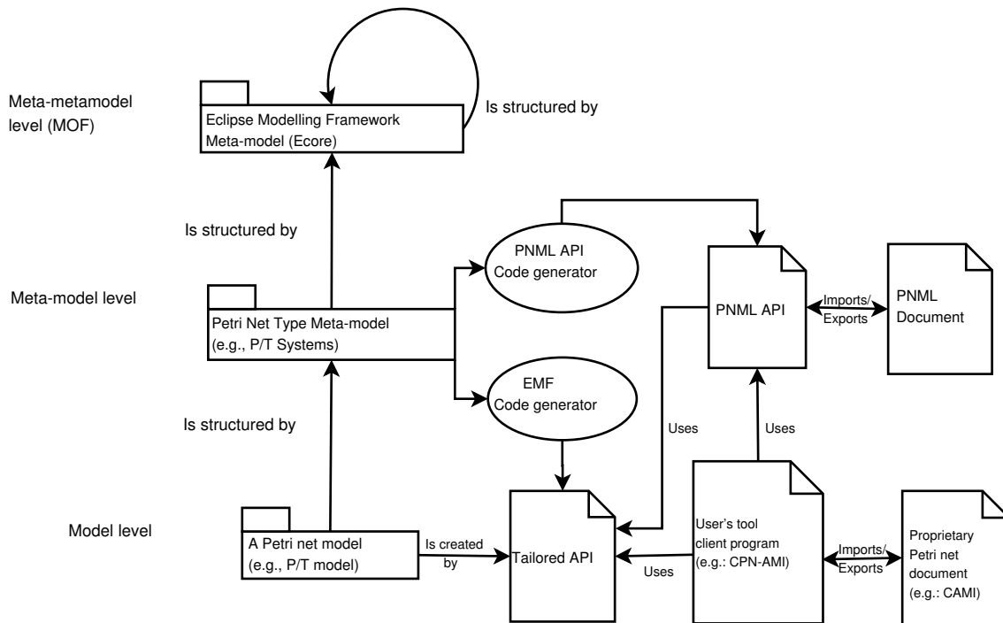
Figure 6: The production chain
