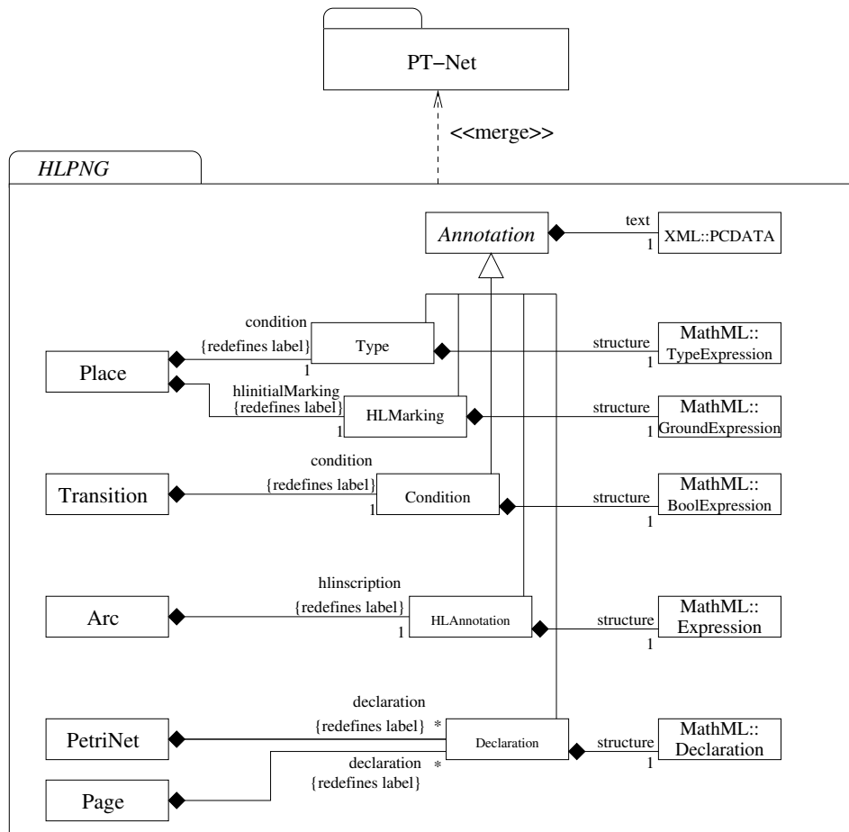
Figure 4: The package HLPNG
