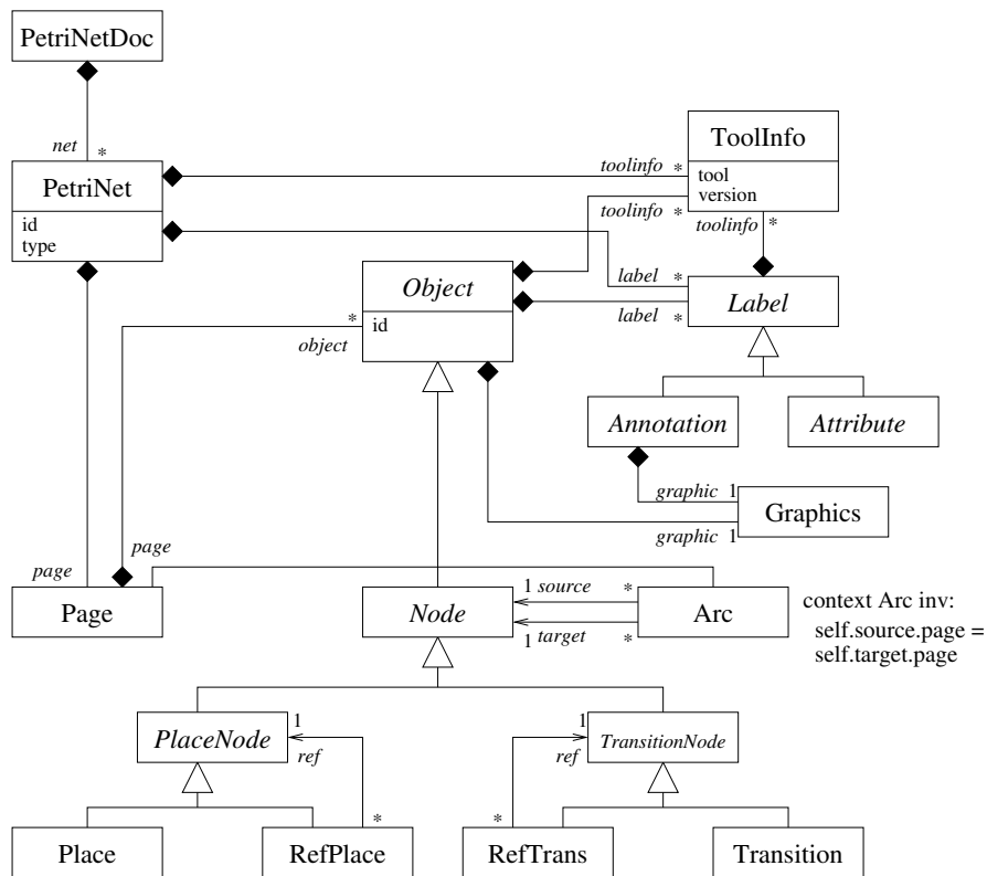
Figure 2: The PNML Core Model
