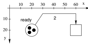
Figure 5: A simple Place/Transition Net
