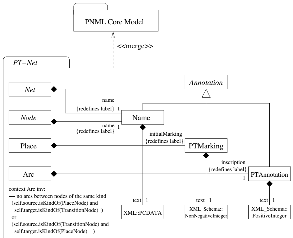
Figure 3: The package PT-Net
