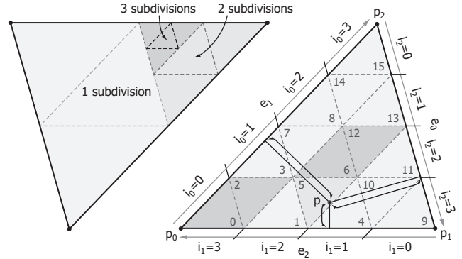
Fig. 6 Our indexing scheme for a volumetric layer.
