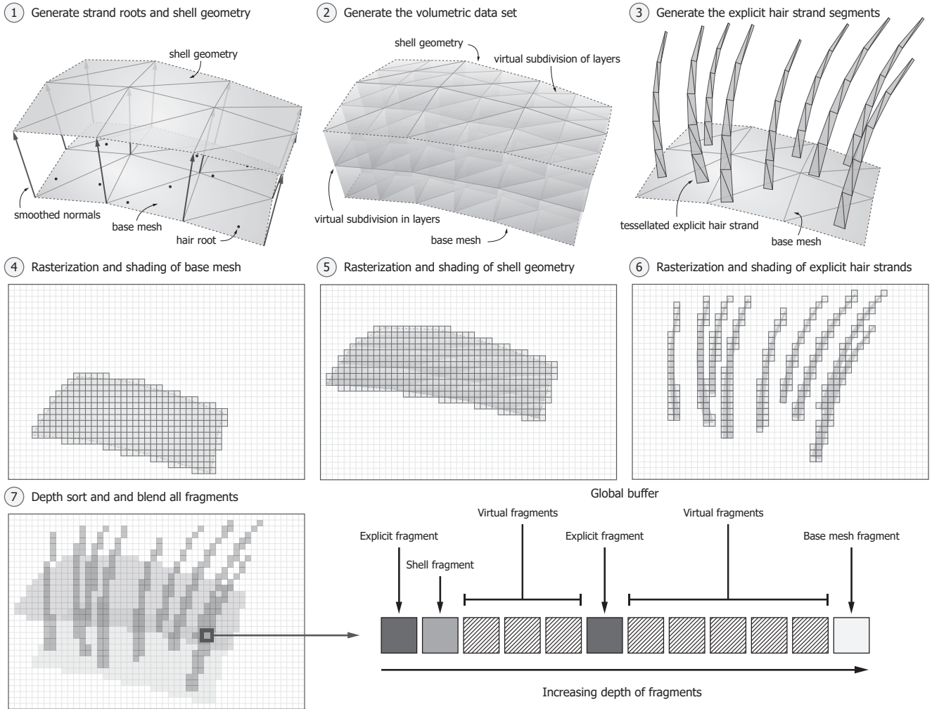
Fig. 3 Overview of our shader pipeline. In steps 1–3, we generate explicit hair strand and shell geometry. In steps 4–6, the generated geometry is rasterized and shaded (see also Fig. 4 and Section 3.1-3.2). In step 7, the shaded fragments are depth sorted and blended in accordance with our blending algorithm (see also Fig. 5 and Section 3.3).
