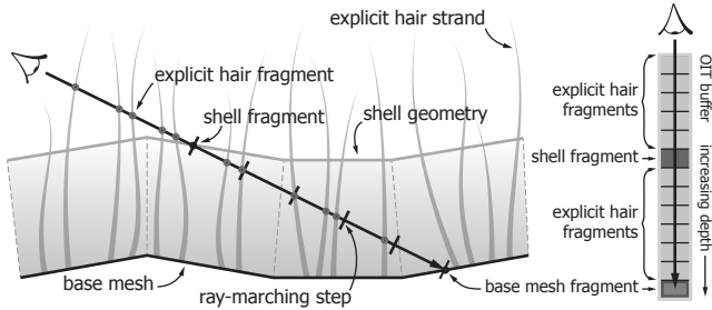
Fig. 5 The fragments generated by the three rasterization steps of our pipeline, seen from the side.
