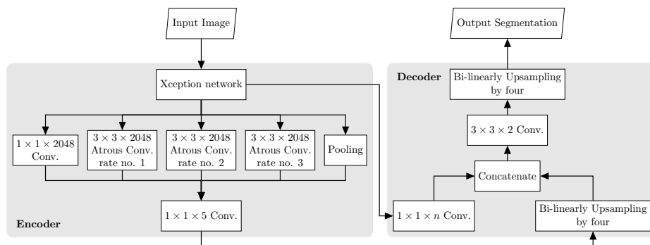
Fig. 4. Illustration of the semantic segmentation network.
