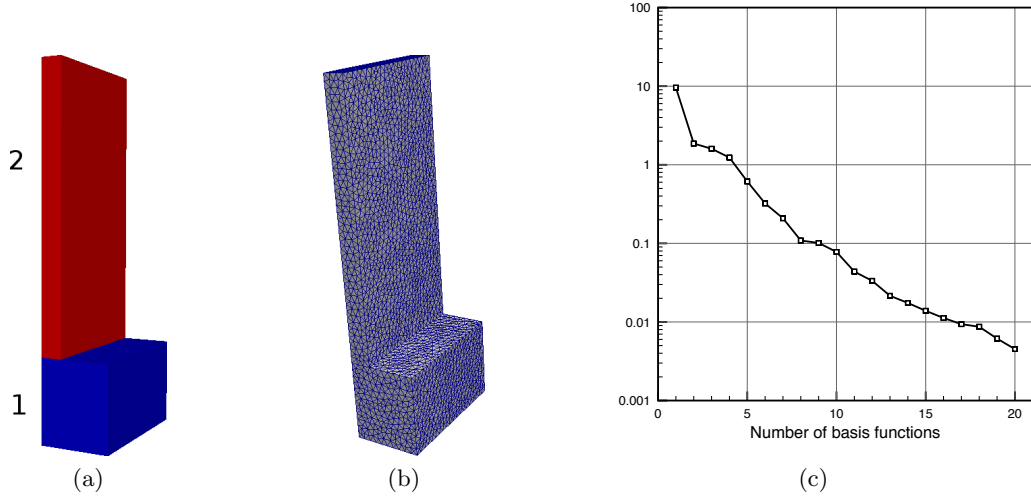
Fig. 6.9: The subdomain division (a), the finite element mesh used for the truth solver (b) and the maximum error over \mathbb{P}_h of the greedy-algorithm with respect to the number of basis functions employed (c) for the thermal fin problem with a geometric parametrization.
