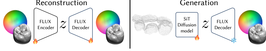
Fig. 3. Overview of CrownFusion. Left: VAE reconstruction from geometry images. Right: conditional generation via SiT diffusion in the learned latent space.
