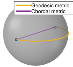
Figure 3. The chordal metric on \mathbb{S}^2 \subset \mathbb{R}^3 is measured directly in \mathbb{R}^3 , while the geodesic metric is measured along \mathbb{S}^2 . Shortest paths with respect to the two metrics coincide, but the chordal metric is not a geodesic metric, and the shortest path is not a geodesic for the chordal metric, because the shortest path between two points is longer than their chordal distance.
